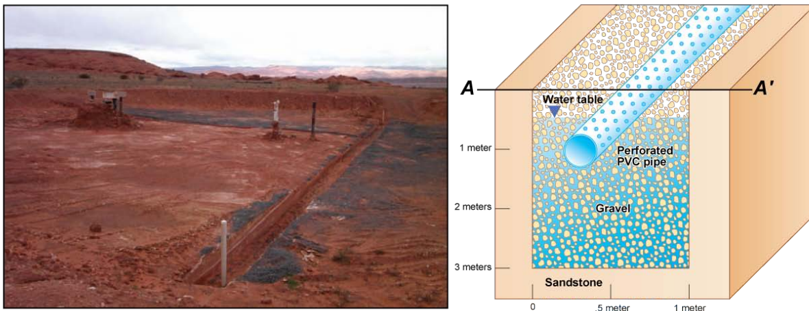
Photo (left) and cross-section (right) of the infiltration trench site at Sand Hollow, southwestern Utah.
